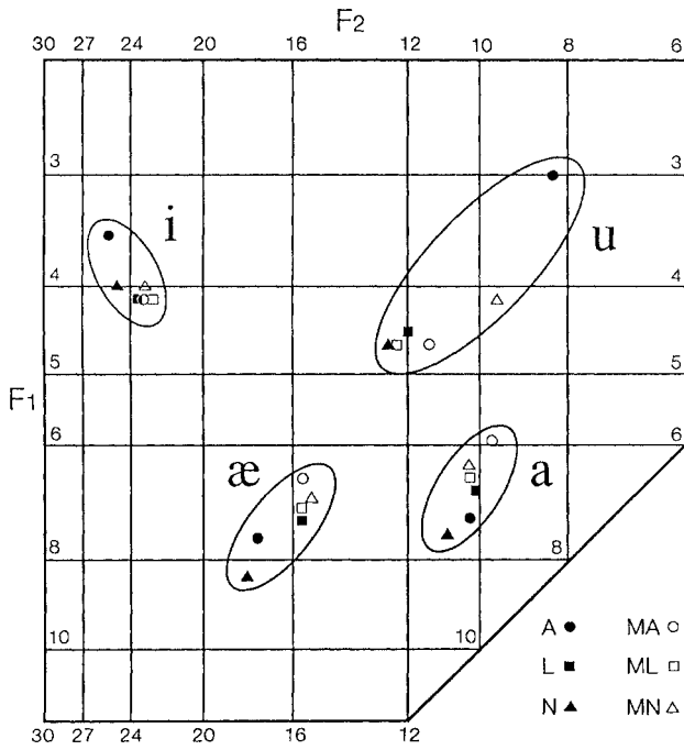
Fig. 1. Vowel space as defined by the frequencies of the first formant (vertical axis) and the second formant (horizontal axis). Frequency is given in hundreds of Hz.
