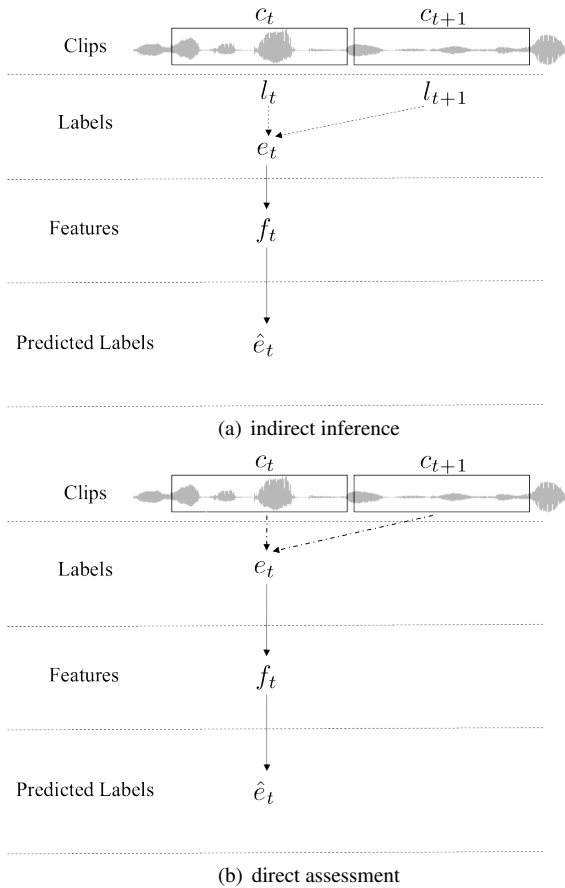
Figure 1: Diagram of labeling and detecting the conflict escalation (a) indirect inference and (b) direct assessment.
