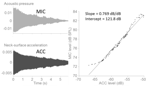
Figure 2: Illustration of the participant-specific calibration of accelerometer (ACC) signal level to sound pressure level from microphone (MIC) signal using the loud-to-soft /a/ vowel task.
