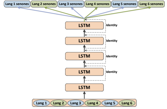
Figure 1: The architecture of SHL-MLSTM with/without residual learning.
