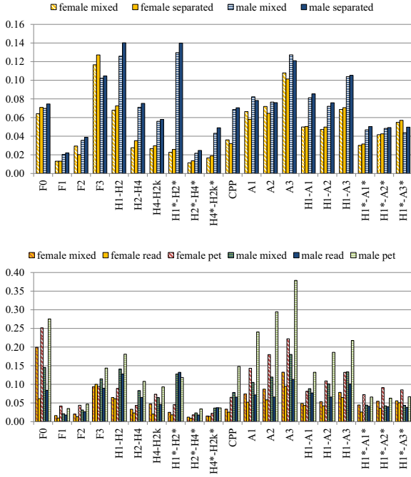
Figure 1: Computed F-ratios of various voice quality features using the UCLA Speaker Variability Database for content (top) and style (bottom) variability. “Separated” in the top panel indicates the subsets were separated by sentences. “Read” and “pet” in the bottom panel indicate the subsets only contained read sentences or pet-directed speech.
