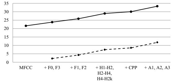
Figure 2: Computed J-measures of VQual2 and MFCC features using read sentences (solid line). Each point on the chart is the J-measure of all features below and to the left of that point. The dashed line shows VQual2 features without MFCCs for comparison.
