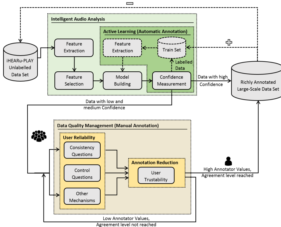
Figure 1: iHEARu-PLAY 's interaction between the intelligent audio analysis, the active learning, and the data quality management components, including the user reliability calculation and the annotation reduction components [6].
