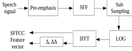
Figure 1: Block diagram of SFFCC extraction.
