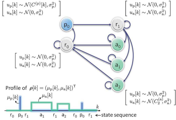
Figure 1: Command function modeling with an HMM.
