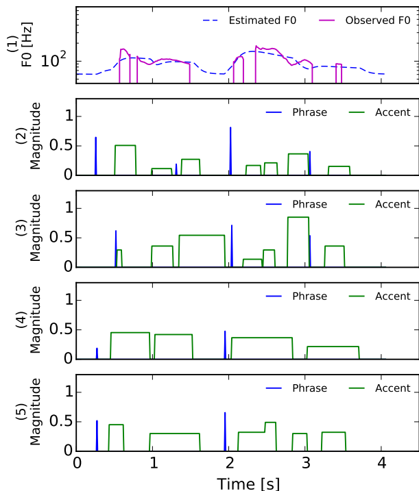
Figure 3: Example of command detection. (1) An observed F_0 contour in voiced regions (solid line) and the estimated F_0 contours by the proposed method (dotted line). The estimated phrase and accent commands. (2) Narusawa’s method [11]. (3) SPACE [17]. (4) DNN-SPACE (the proposed method). (5) Grand truth (manually labeled by an expert).
