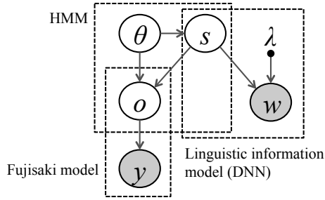
Figure 2: Graphical representation of proposed model.
