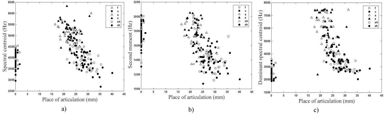
Figure 3: Relationship between the spectral parameters and the place of constriction for voiced /v, z, ʒ/ and unvoiced /f, s, ʃ/ fricatives: (a) spectral centroid, (b) standard deviation, (c) dominant spectral centroid.
