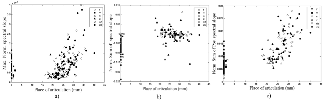
Figure 4: Relationship between spectral parameters and place of articulation for voiced /v, z, ʒ/ and unvoiced /f, s, ʃ/ fricatives: (a) maximum normalized spectral slope, (b) normalized sum of spectral slope, (c) normalized sum of positive spectral slope.
