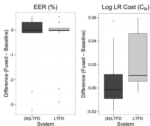
Figure 1: Distributions of raw EER (L) and C_{llr} (R) differences between the fused systems using (M)LTFDs and LTFDs and baseline MFCC system.
