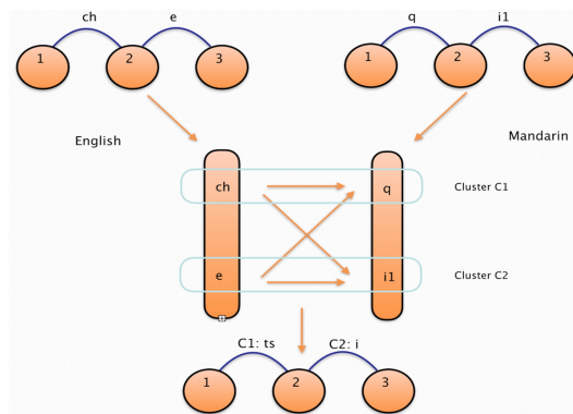
Figure 1: Goal of the system: from English-Mandarin dynamic alignments to bipartite graph for clustering and constructing the predicted transcription labels. The sentence is from the real example in Table 2.
