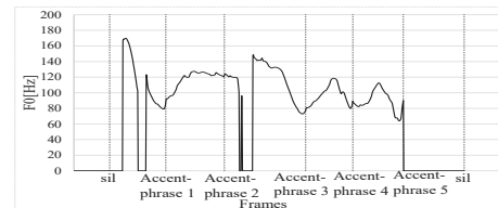
Figure 4: Smoother f0 sequences by chunk connection.
