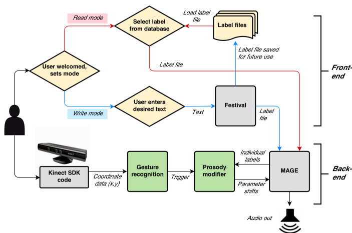
Figure 1: System setup.
