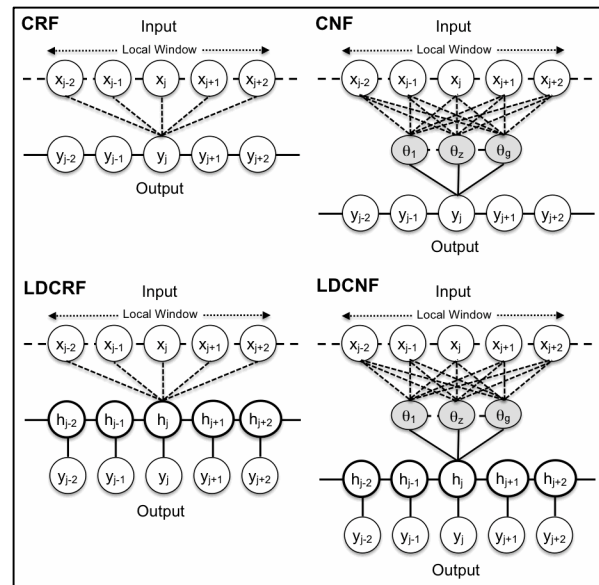
Figure 1. The various PGM considered in this study. The gate units \theta_1 \dots \theta_g are in gray while the hidden units h_1 \dots h_n present a thick border. For clarity, only the region of the model net surrounding the generic input feature vector x_j is represented in the pictures.
