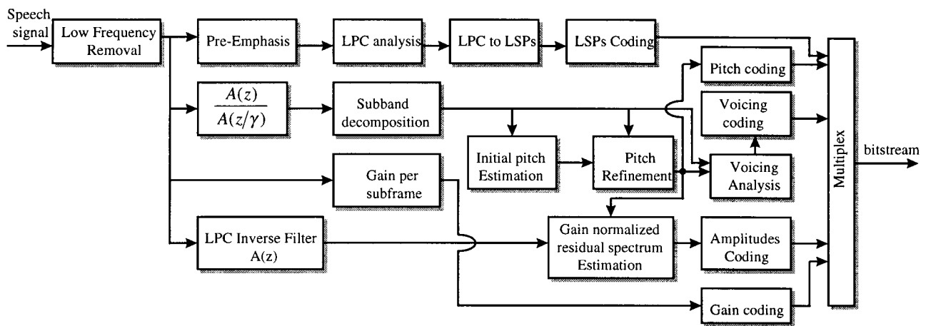
Figure1: Block diagram of the coder
